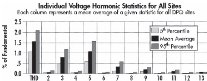
Figure 24: Individual Voltage Harmonic Statistics 222 EPRI DPQ Sites from 6/1/93 to 6/1/94
