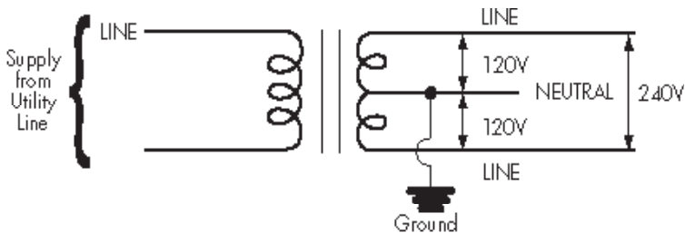
Figure 4: 120/240 V Single-phase Service
