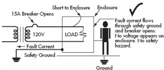
Figure 11: Equipment with Proper Equipment Bonding
