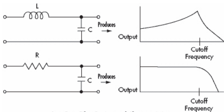
Figure 27: Examples of Untuned Filters
